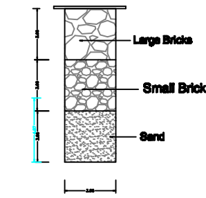
SECTION OF RAIN WATER COLLECTION PITS (NTS) RWL CAPACITY = 2000 LTR
