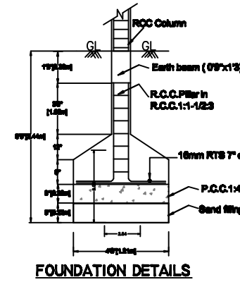
FOUNDATION DETAILS
