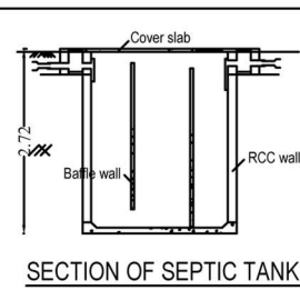
SECTION OF SEPTIC TANK
