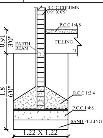
FOUNDATION DETAILS (NOT TO SCALE)
