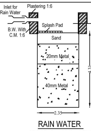
RAIN WATER PERCOLATION PIT
