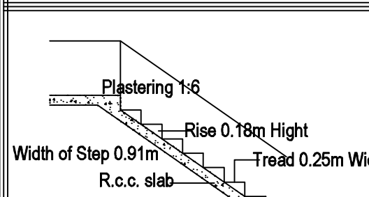
DETAILS OF STAIR CASE
