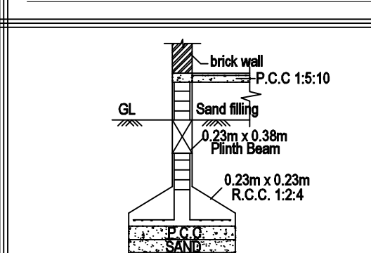
→ 0.99 ← FOUNDATION DETAILS
