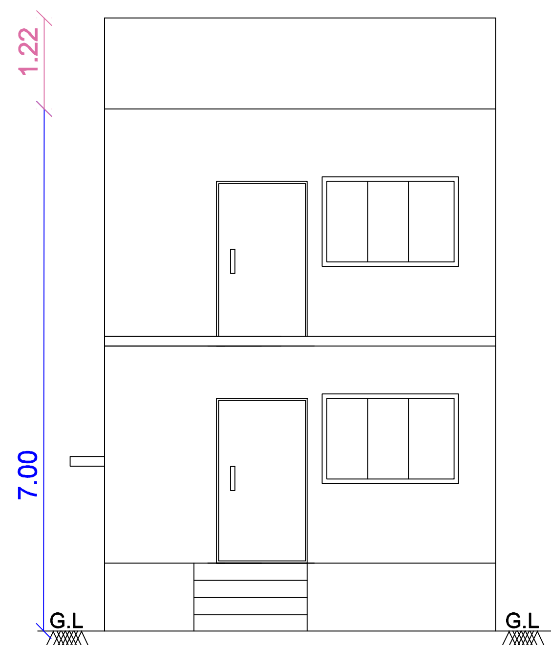
FRONT ELEVATION
