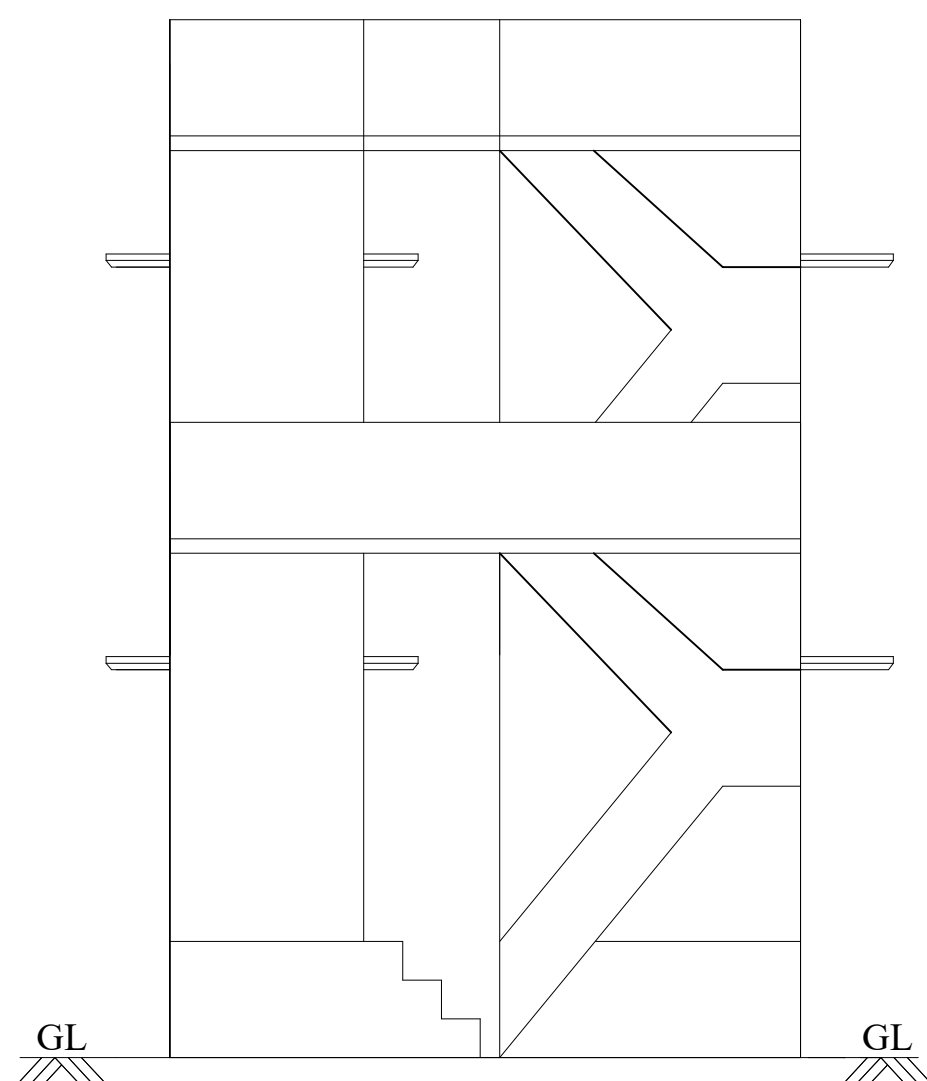
FRONT ELEVATION
