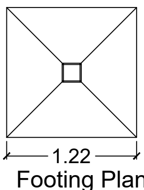
Footing Plan
