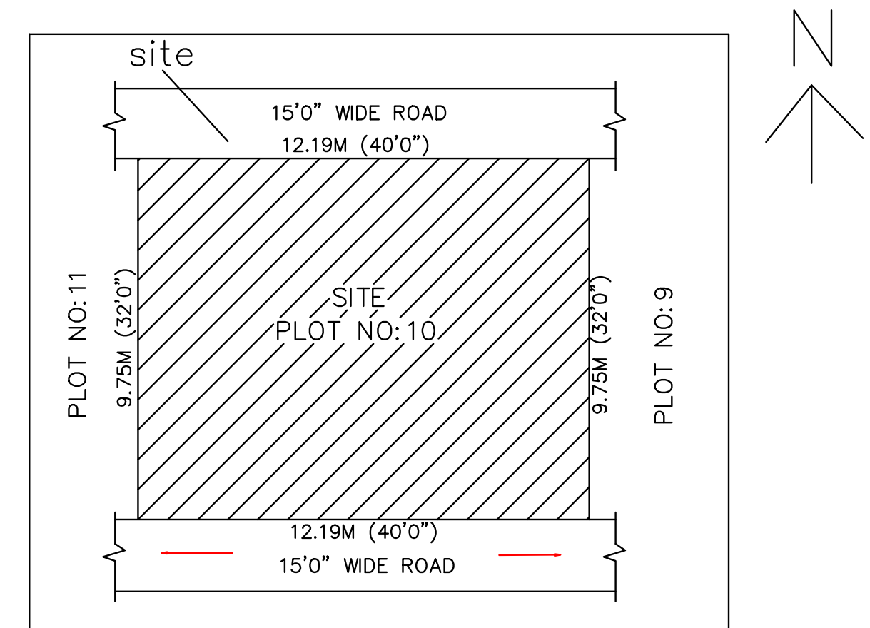
SITE PLAN
