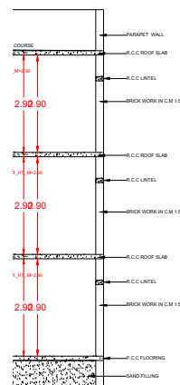
SECTION
