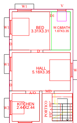
PROPOSED GROUND FLOOR N
