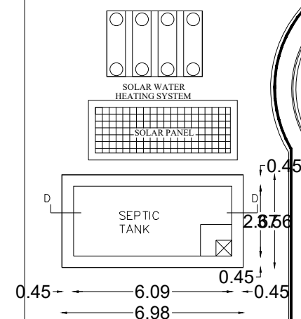
PLAN OF SEPTIC TANK SCALE 1"=2'0"
