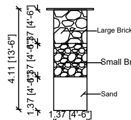
SECTION OF RAIN WATER
