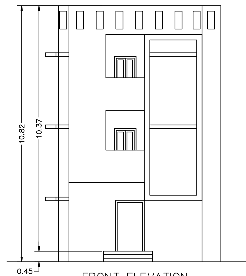
FRONT ELEVATION
