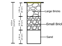
SECTION OF RAIN WATER COLLECTION PITS (NTS)
