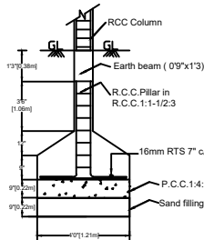
FOUNDATION DETAILS
