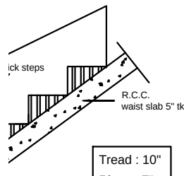
TAIRCASE DETAILS-nts
