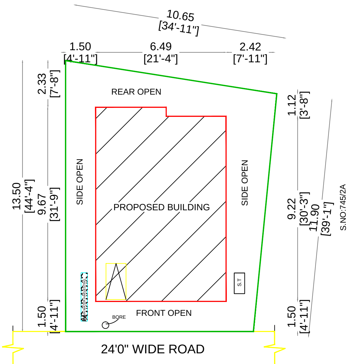
9.35 [30'-8"] SITE PLAN
