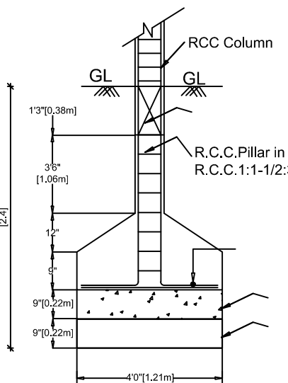
FOUNDATION DETAILS
