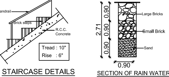
STAIRCASE DETAILS
