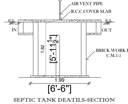
SEPTIC TANK DETAILS-SECTION
