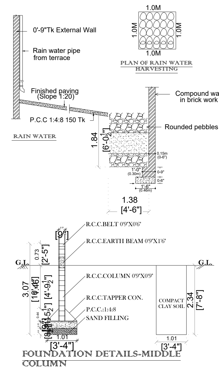
FOUNDATION DETAILS-MIDDLE COLUMN
