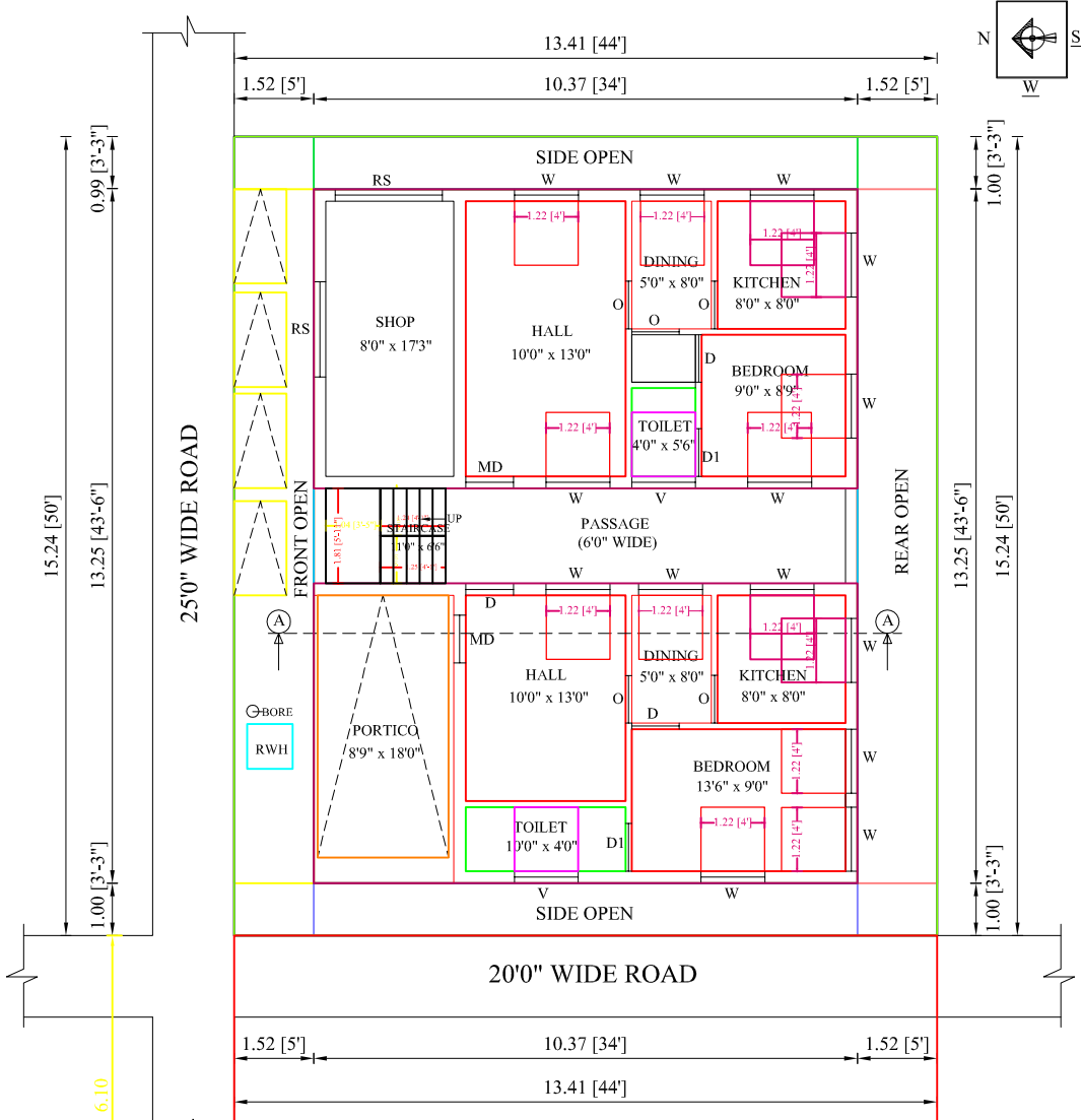
FLOOR PLAN
