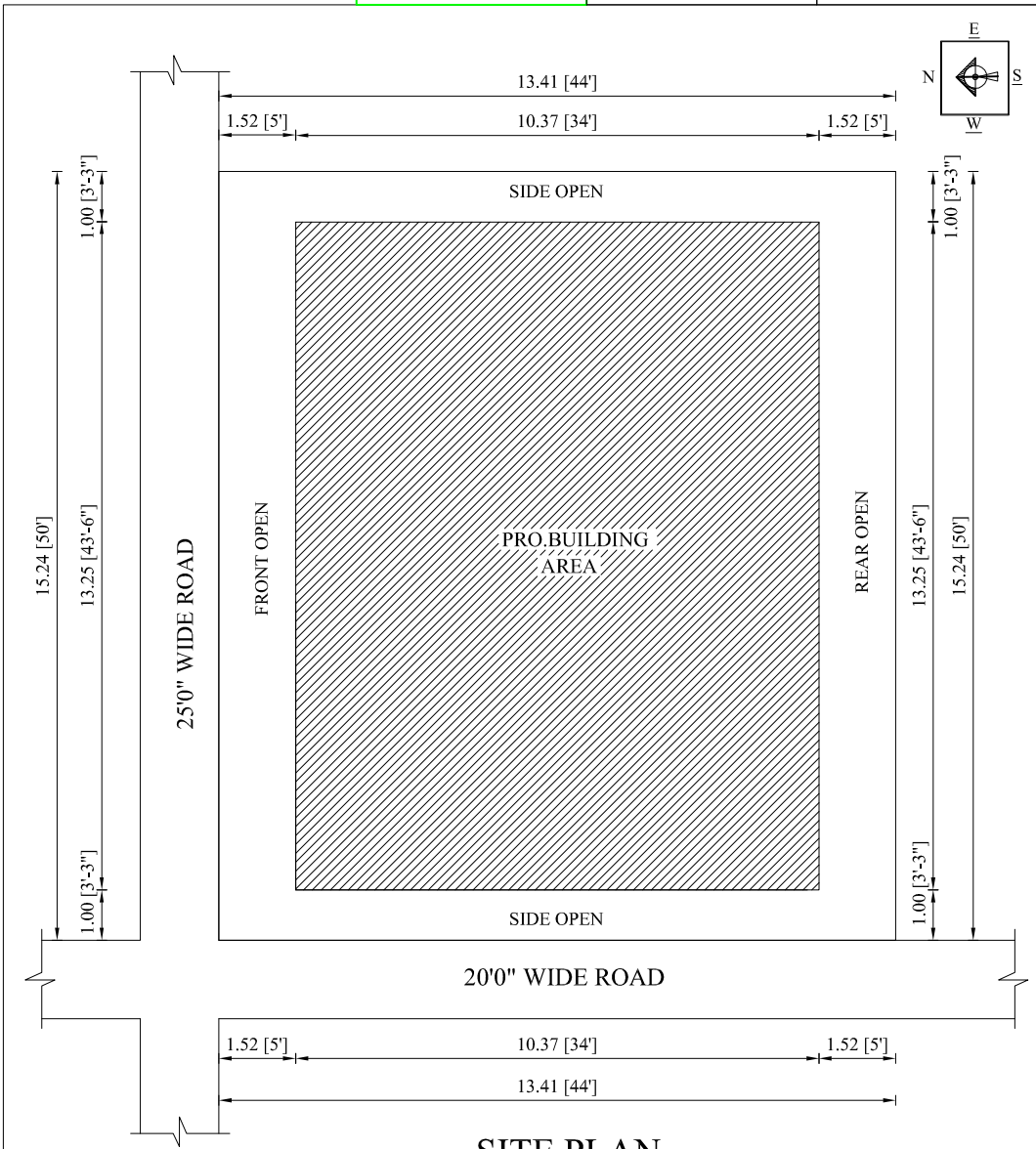
SITE PLAN
