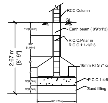
FOUNDATION DETAILS
