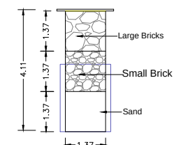
SECTION OF RAIN WATER COLLECTION PITS (INTS)
