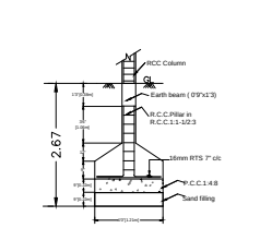
FOUNDATION DETAILS
