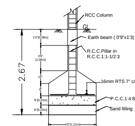
FOUNDATION DETAILS
