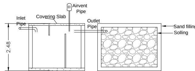
SECTION
