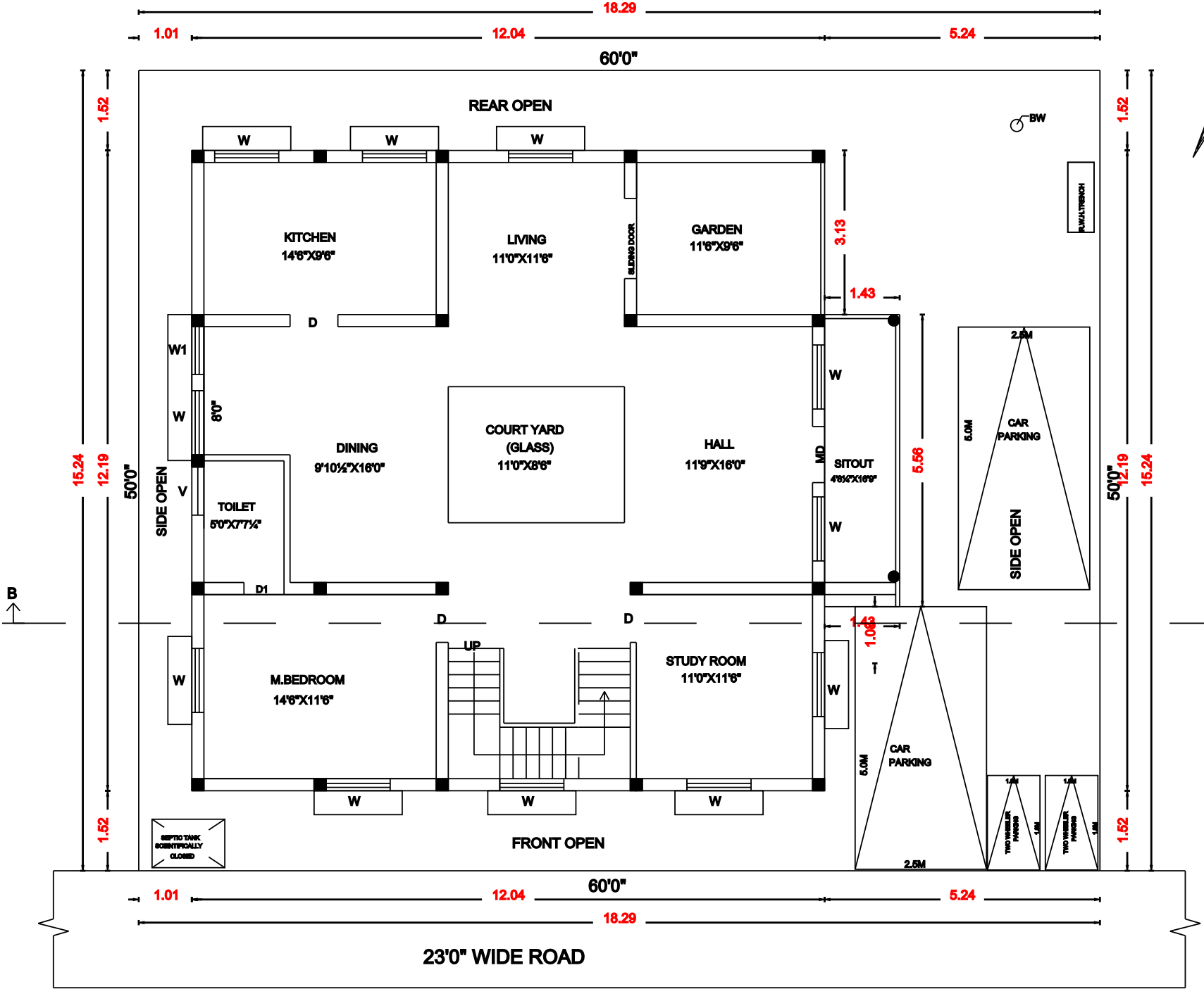
PRO.GROUND FLOOR PLAN
