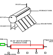
SOLAR HOT WATER SYSTEM DETAILS
