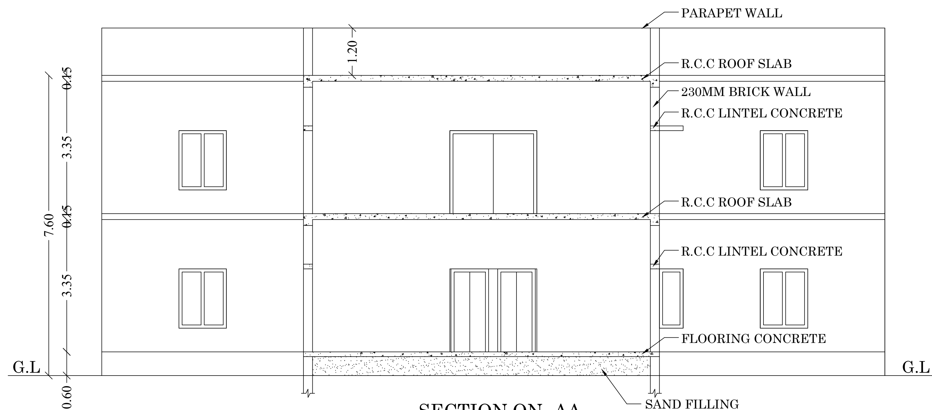
SECTION ON -AA (BLOCK-01)
