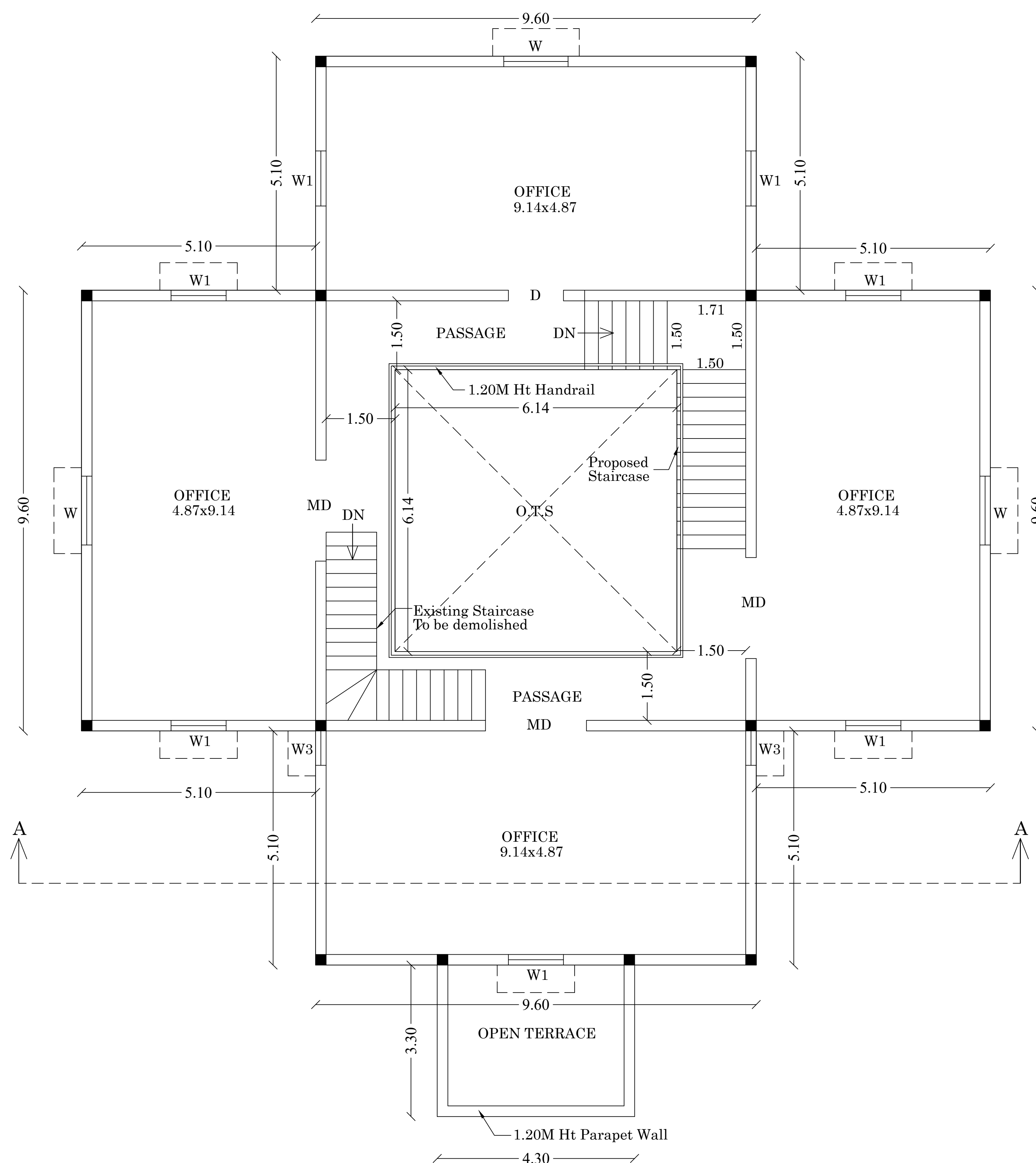
FIRST FLOOR PLAN (BLOCK-01)
