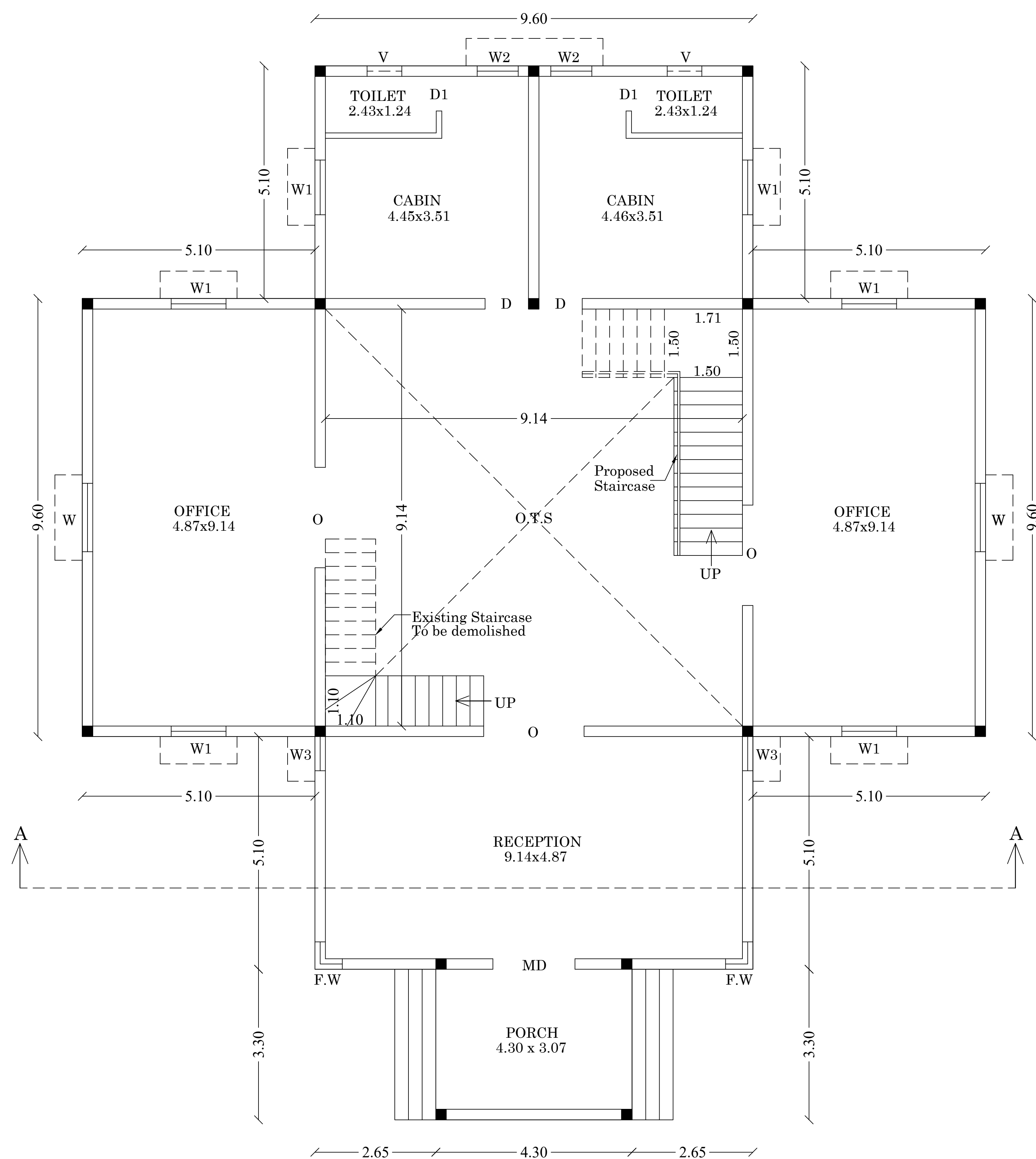
GROUND FLOOR PLAN (BLOCK-01)
