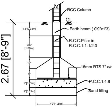
FOUNDATION DETAILS
