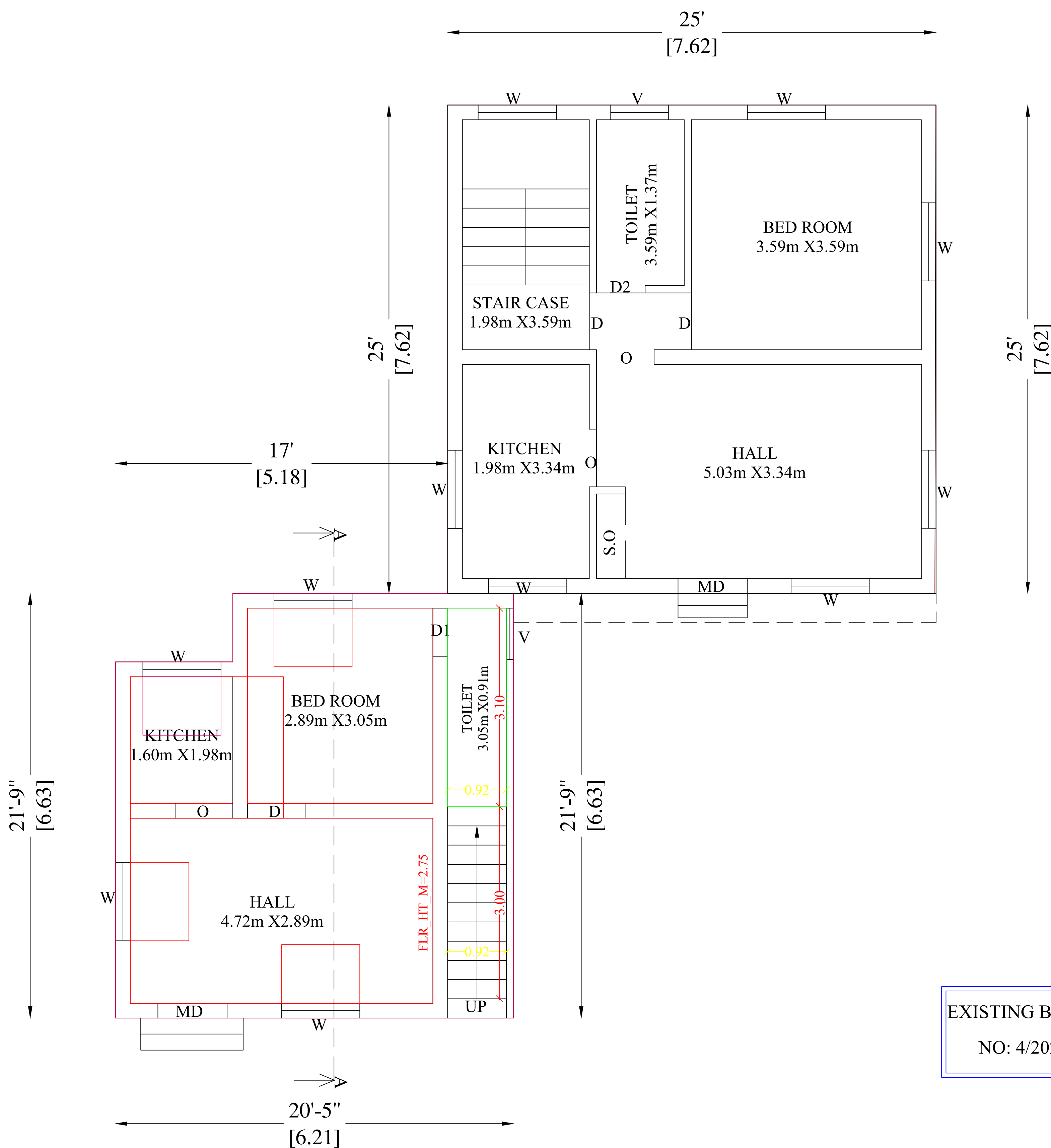
EXG. & PRO. GROUND FLOOR PLAN
