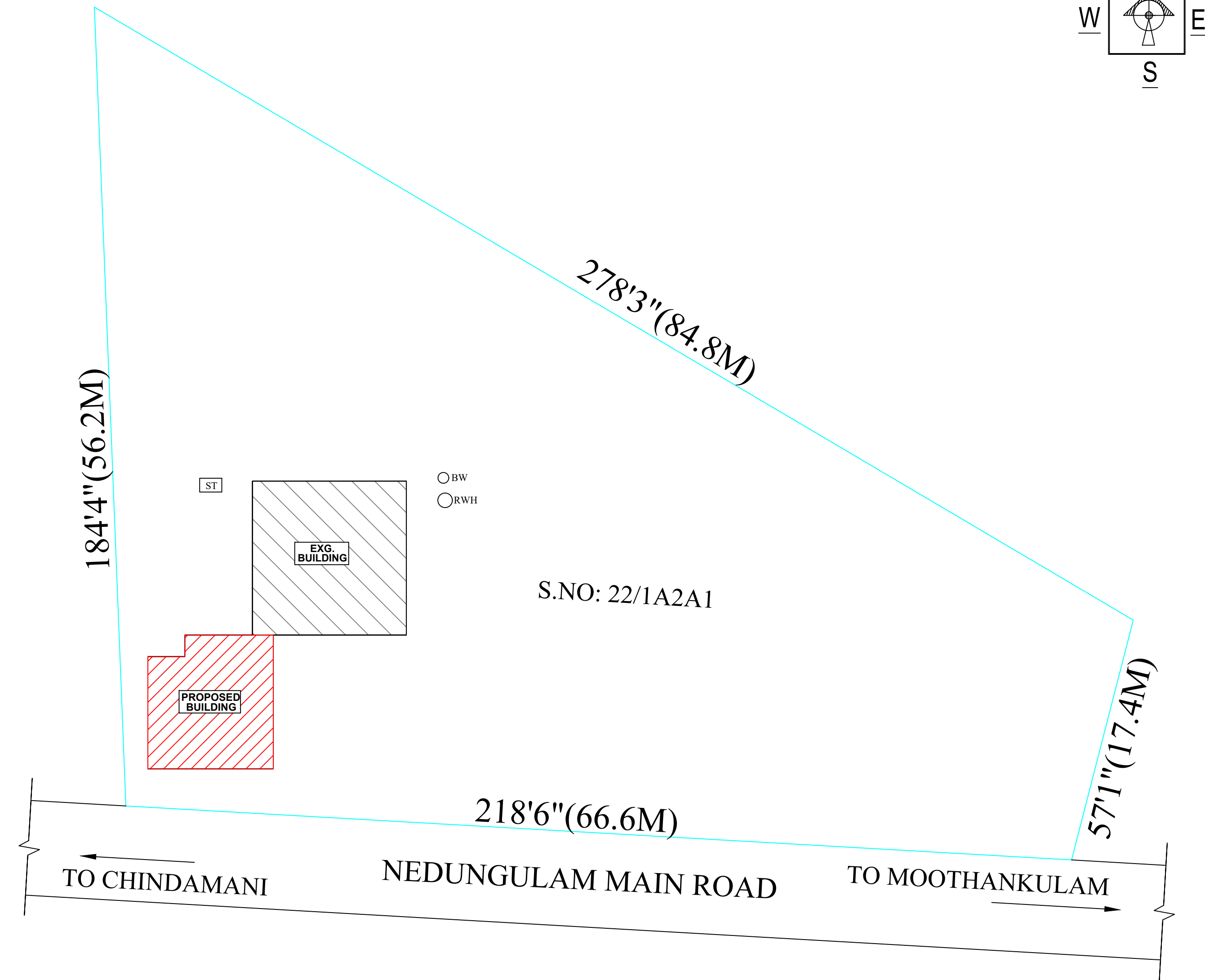
SITE PLAN (AS PER FMB)
