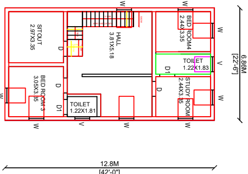
PRO. FIRST FLOOR PLAN.
