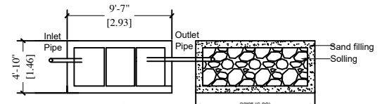
DETAILS OF SEPTIC TANK & DISPERSION TRENCH
