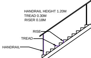
STAIR CASE DETAILS
