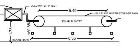
SIDE ELEVATION
