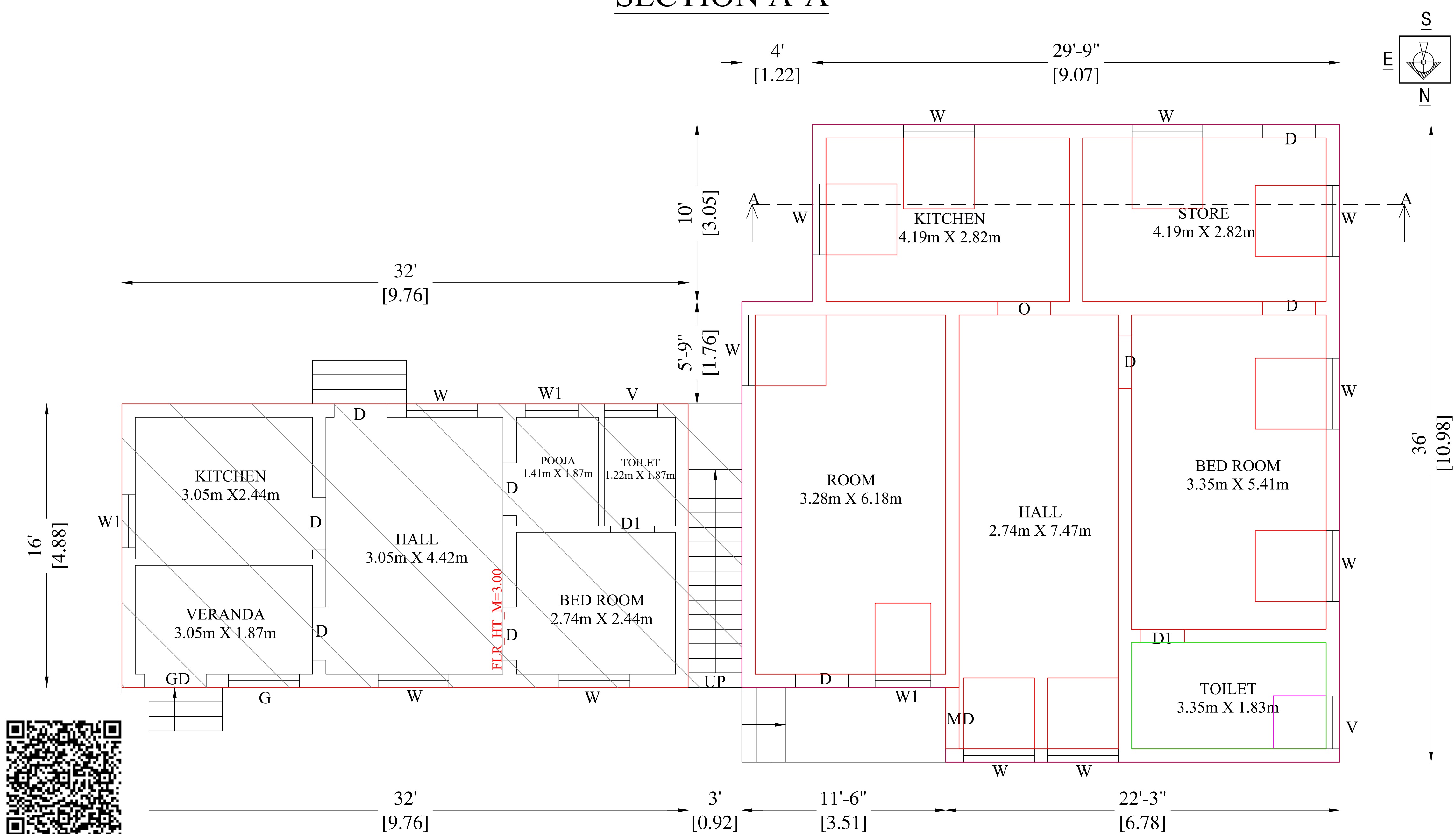
EXG. & PRO. GROUND FLOOR PLAN
