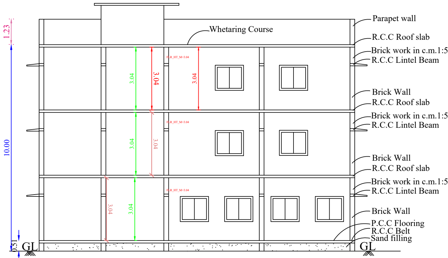
SECTION A'-A'
