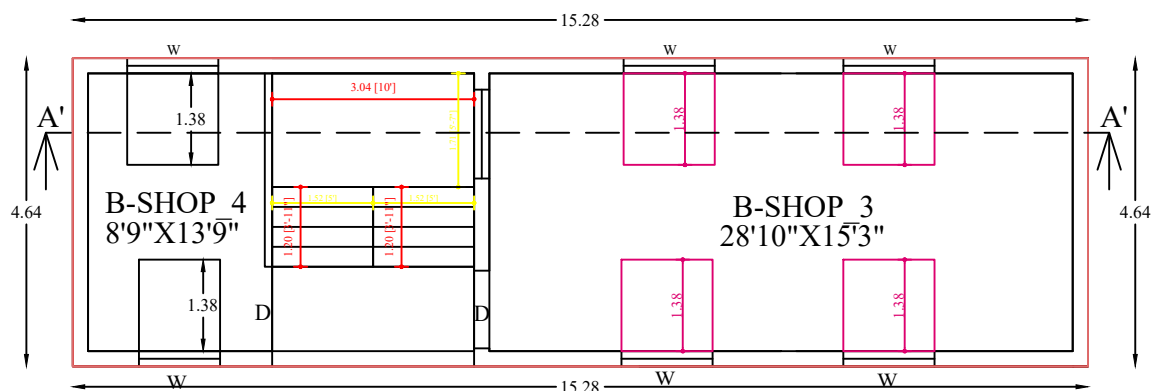
FIRST FLOOR PLAN (EXISTING)
