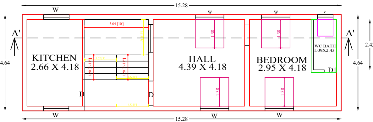
SECOND FLOOR PLAN (PROPOSED)
