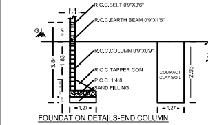
FOUNDATION DETAILS-END COLUMN
