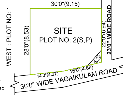
TOPO PLAN (NOT TO SCALE)
