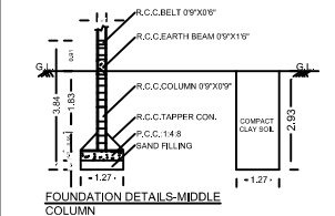
FOUNDATION DETAILS-MIDDLE COLUMN
