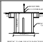
SEPTIC TANK DETAILS-SECTION
