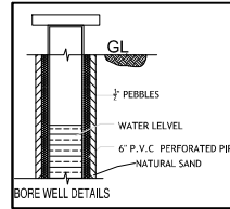
BORE WELL DETAILS
