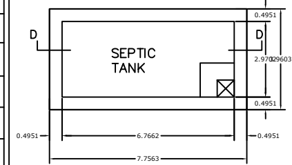
PLAN OF SEPTIC TANK SCALE 1"=2'-0"
