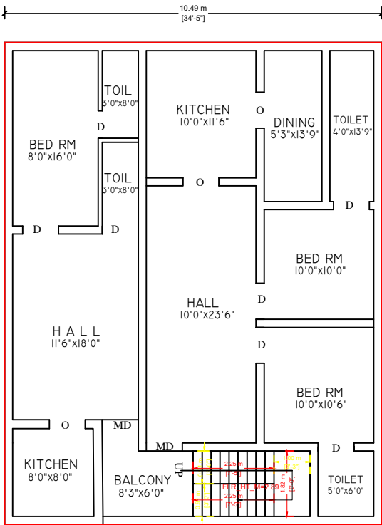
EXG., FIRST FLOOR PLAN
