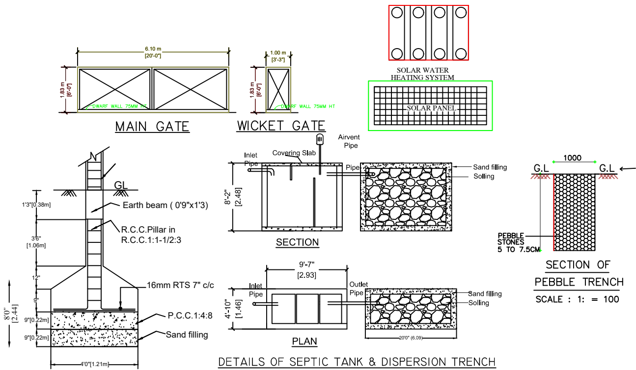
FOUNDATION DETAILS
