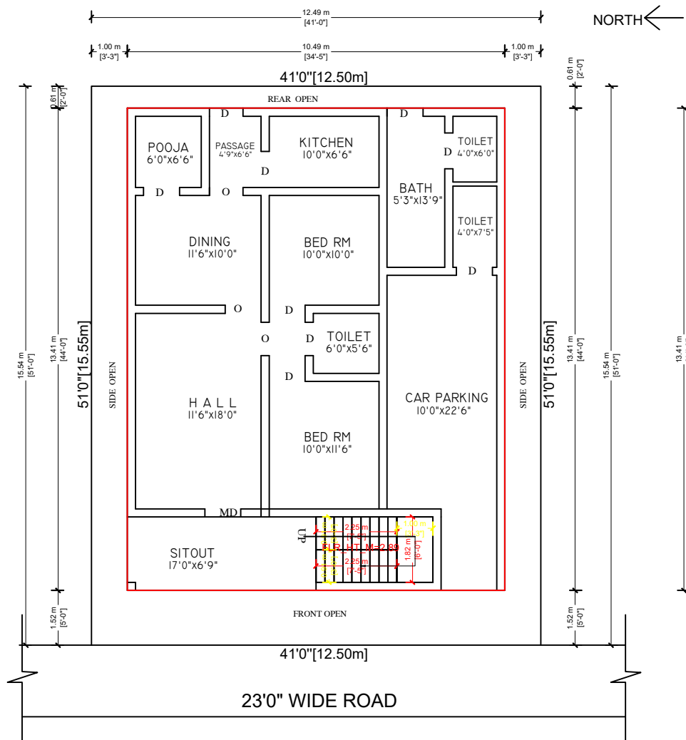
EXG., GROUND FLOOR PLAN
