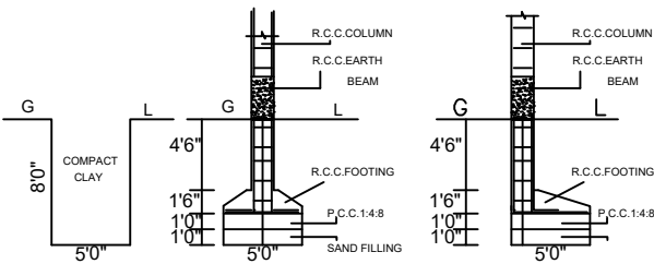
FOUNDATION DETAILS
