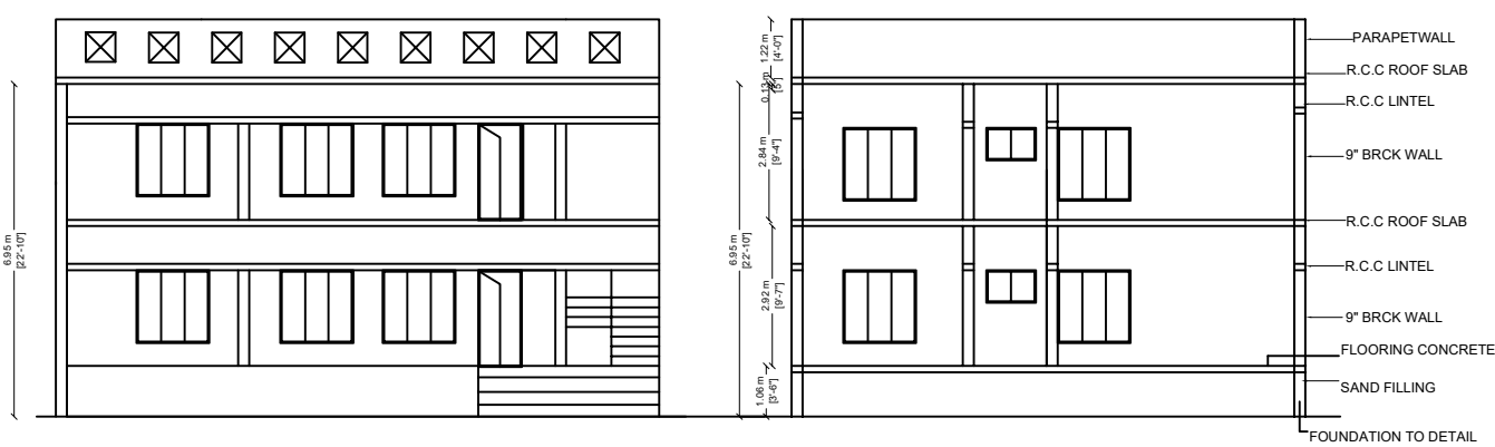
FRONT ELEVATION
