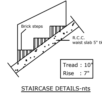
STAIRCASE DETAILS-nts
