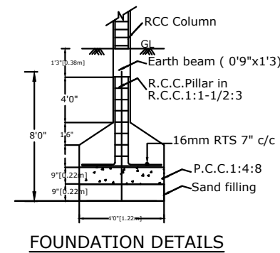
FOUNDATION DETAILS
