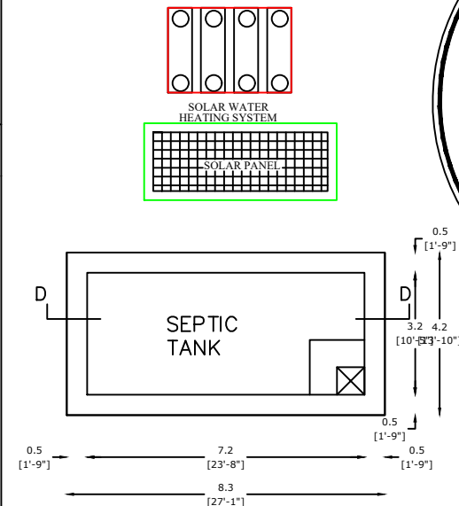
PLAN OF SEPTIC TANK SCALE 1"=2'0"
