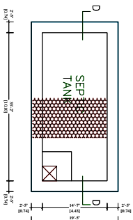
PLAN OF SEPTIC TANK SCALE 1"=2'0"
