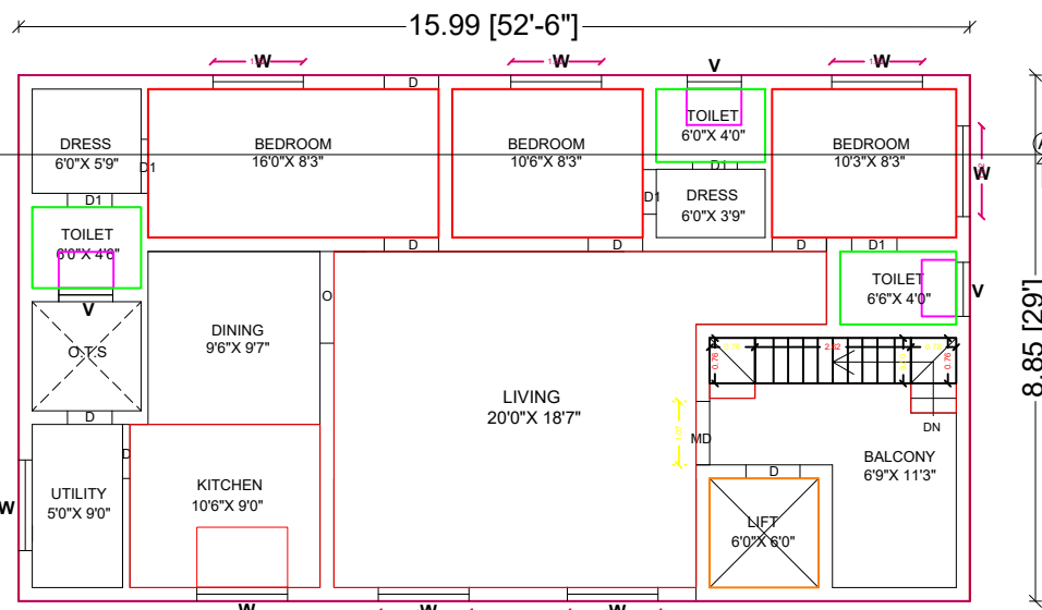
PRO.SECOND FLOOR PLAN
