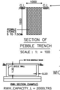
RWH_CAPACITY_L = 2000LTRS
