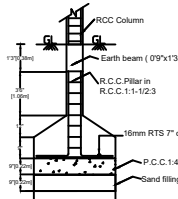
FOUNDATION DETAILS
