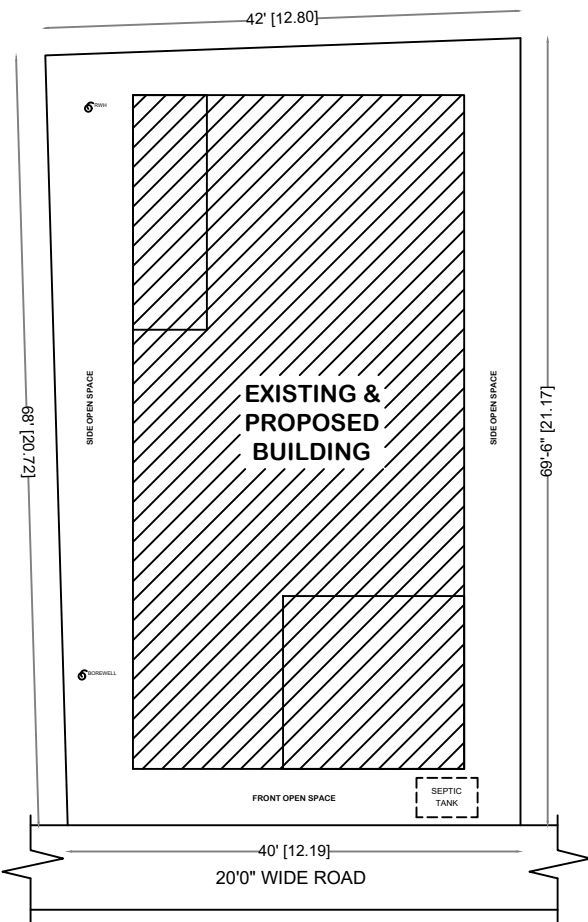
SITE PLAN
