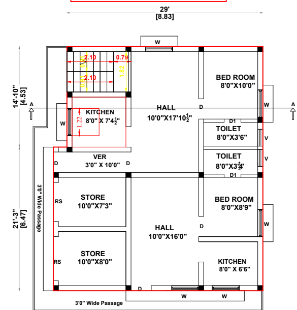
FIRST FLOOR PLAN (EXISTING)
