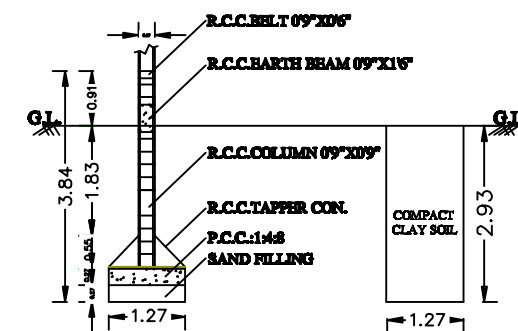
FOUNDATION DETAILS-MIDDLE
