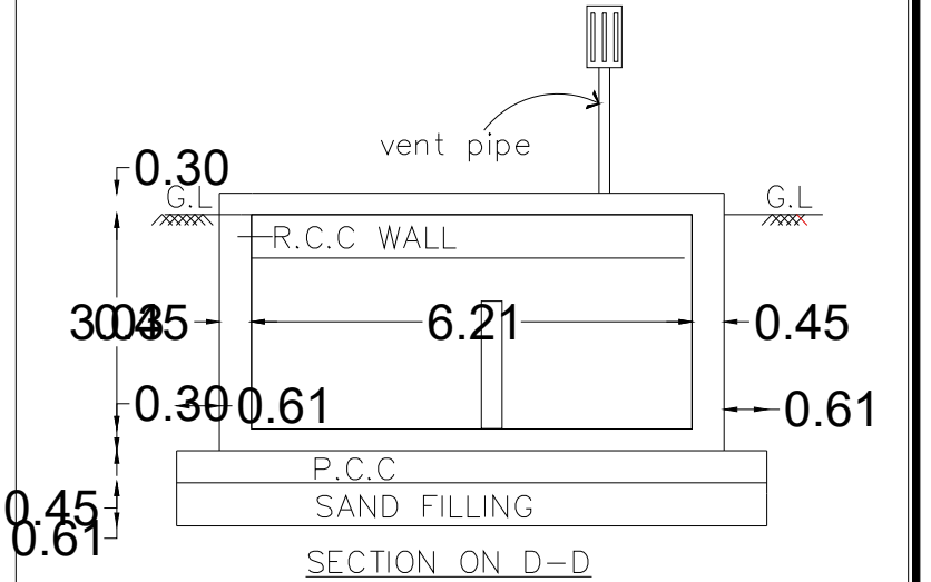
SECTION ON D-D
