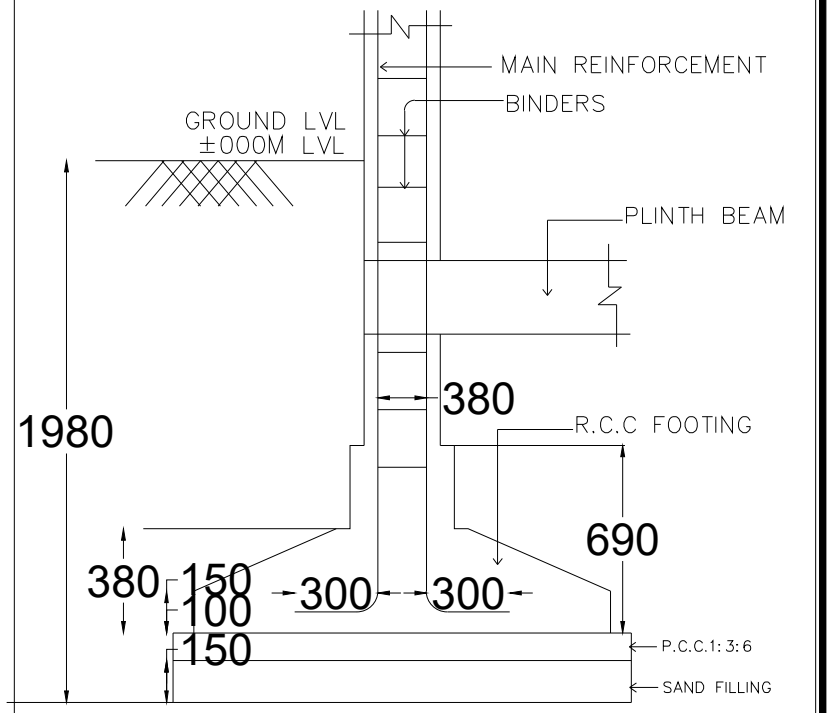
TYPICAL SECTION OF R.C.C COLUMN FOUNDATION SCALE : 1" = 2'-0"
