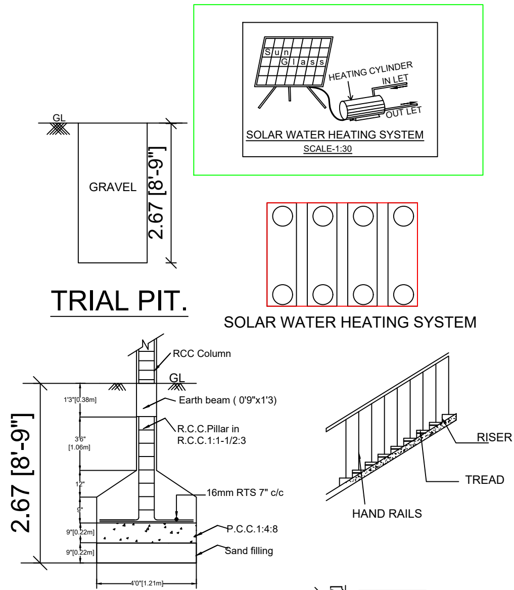
FOUNDATION DETAILS
