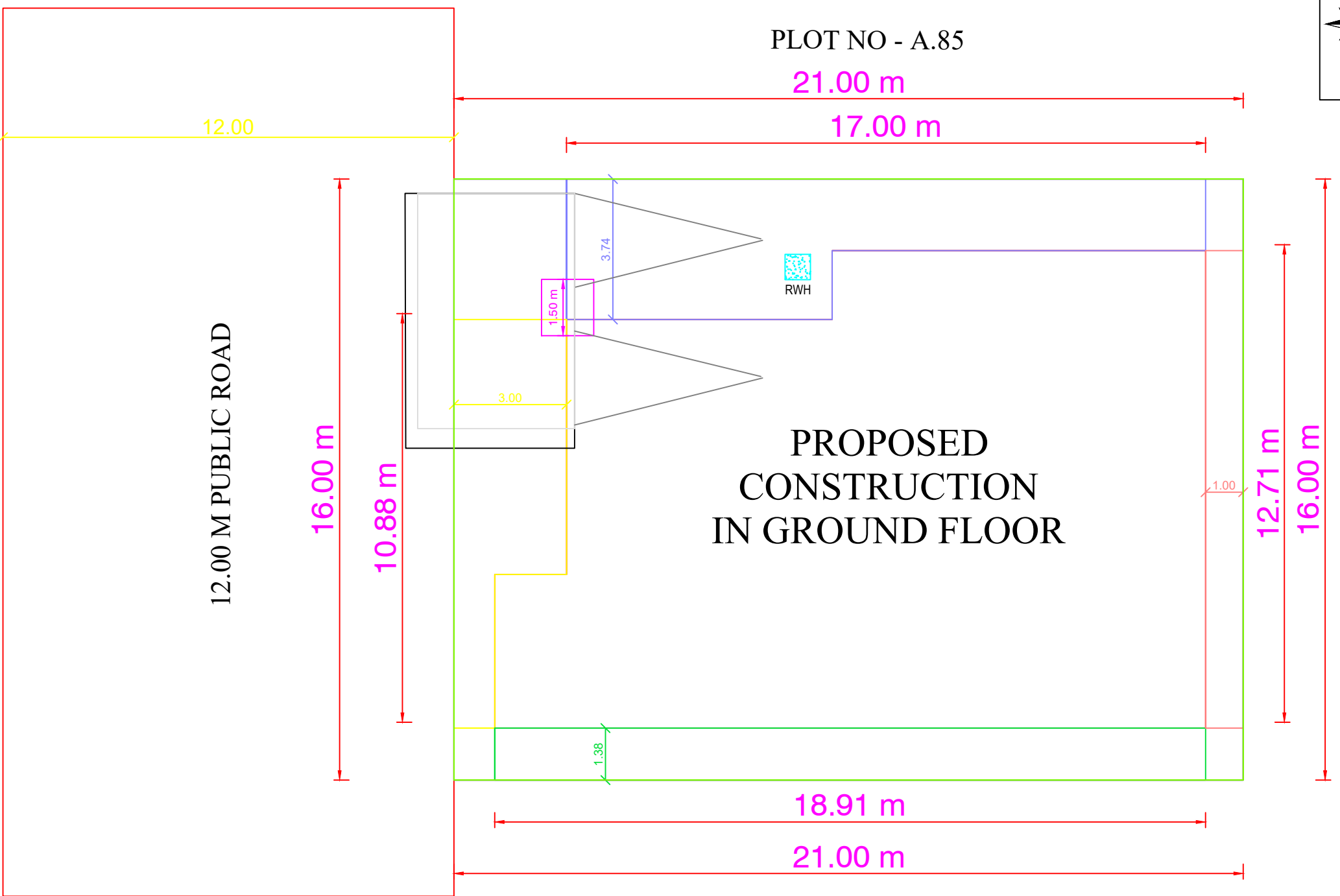
SITE PLAN
