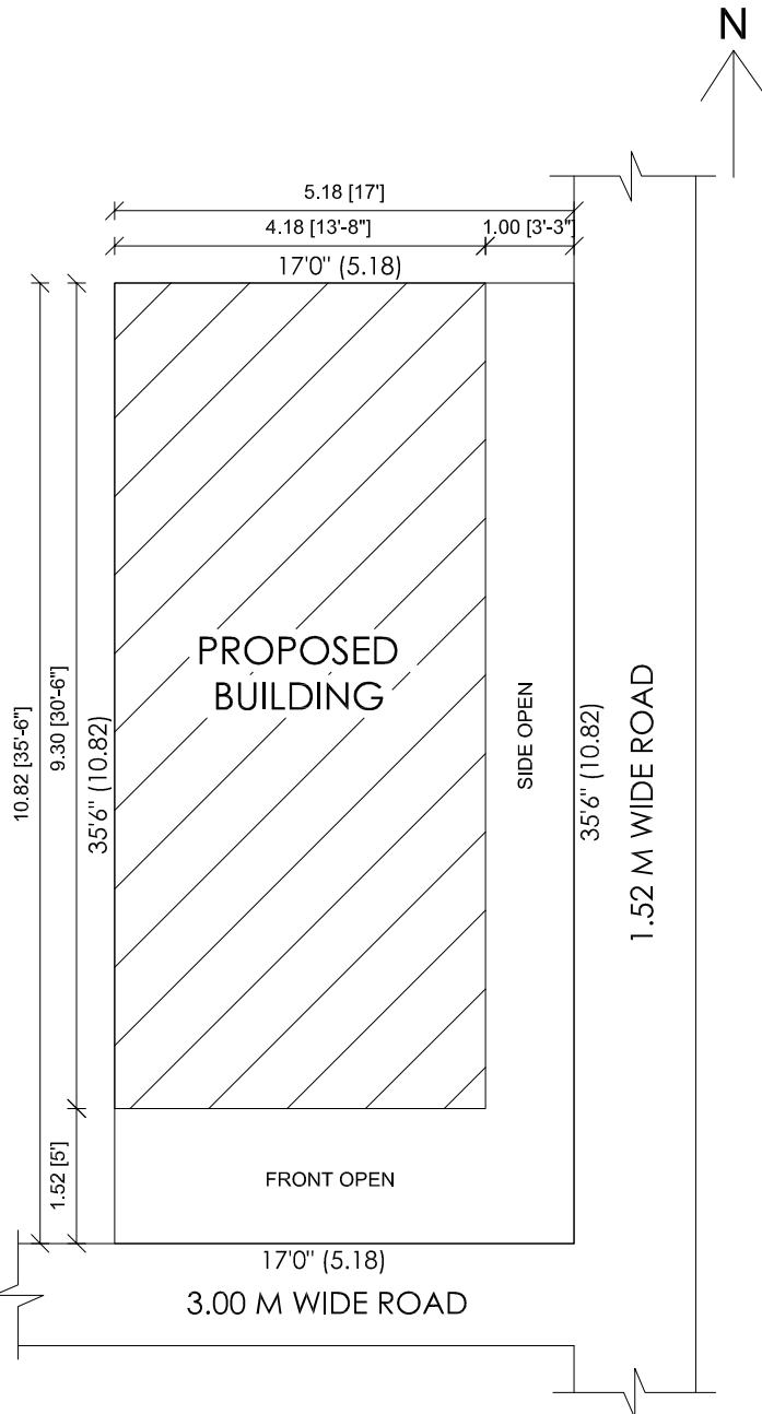
SITE PLAN
