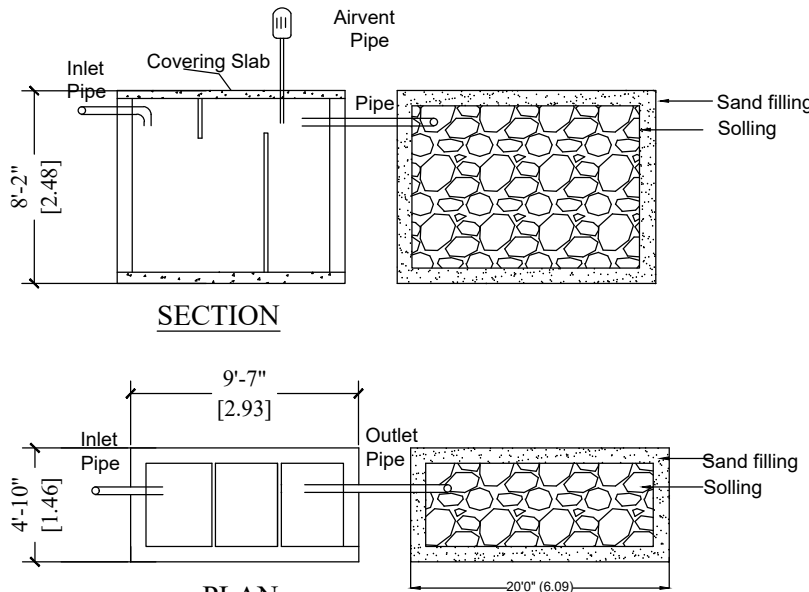
DETAILS OF SEPTIC TANK & DISPERSION TRENCH
