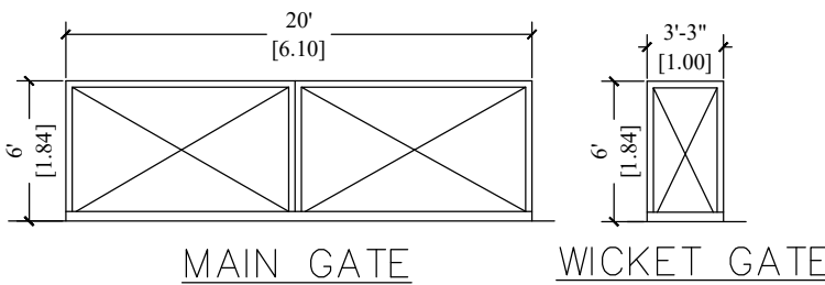
MAIN GATE
