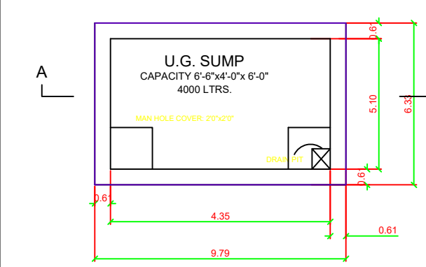
SUMP DETAIL
