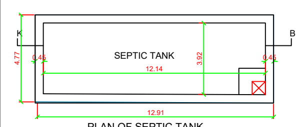
PLAN OF SEPTIC TANK SEPTIC TANK
