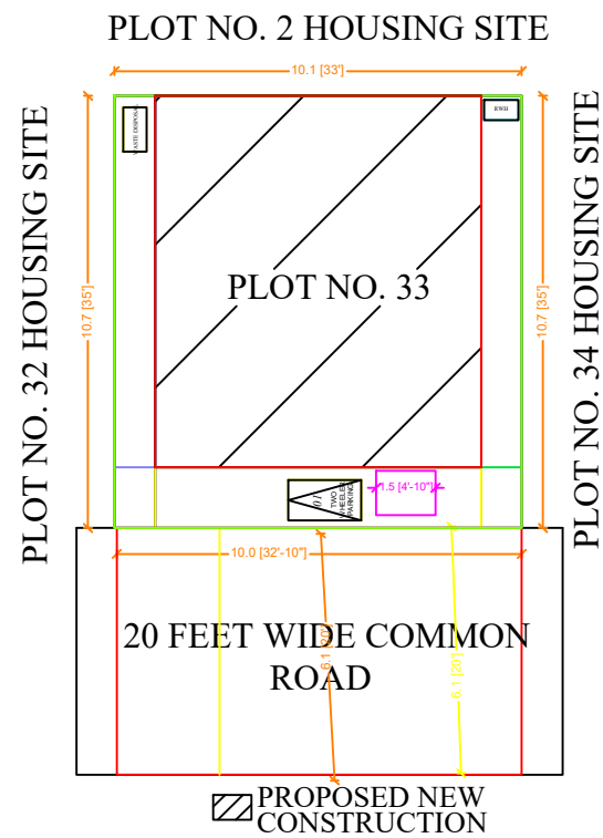
SITE PLAN FOR PLOT NO. 33 (SURVEY NO. 65/7B1C)
