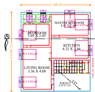
GROUND FLOOR PLAN (1ST DWELLING UNIT)
