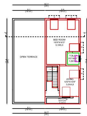
PROPOSED FIRST FLOOR
