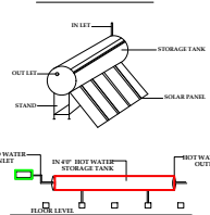
SOLAR HOT WATER SYSTEM DETAILS
