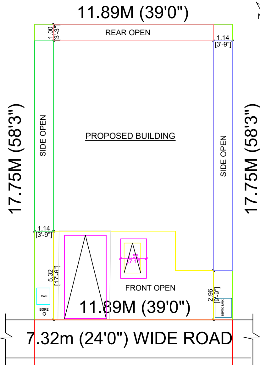
SITE PLAN
