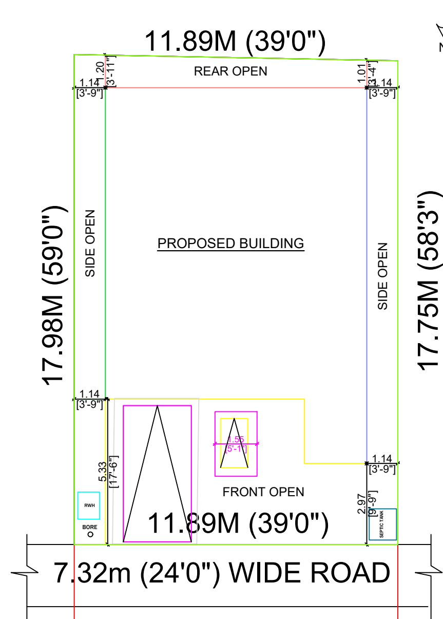
SITE PLAN
